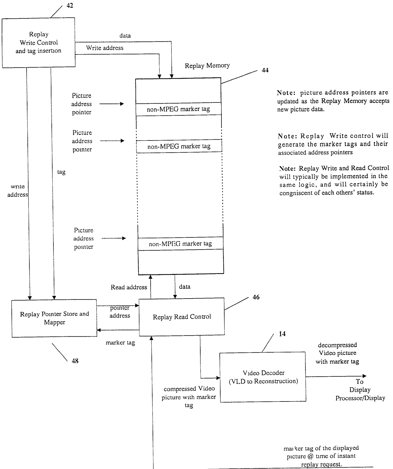
Figure 4: Major Components of the Instant Replay SubSystem
